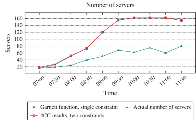
Figure 4. (Color online) Required Staffing to Operate in the QED Regime (Red) vs. Actual Staffing (Blue)
