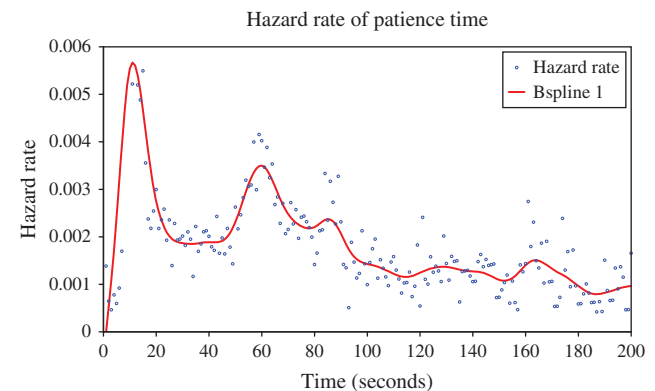
Figure 3. (Color online) Hazard Rates of a Patience-Time Distribution in an Israeli Call Center
