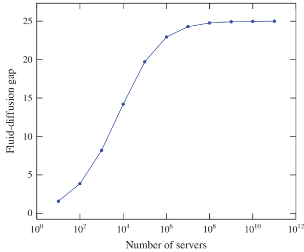
Figure 6. (Color online) Gap Between the Fluid and Diffusion Approximations
