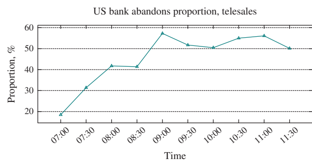
Figure 5. (Color online) Fraction of Abandonment Under Actual Staffing
