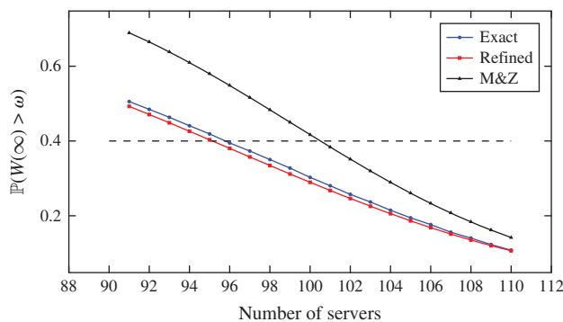
Figure 2. (Color online) Staffing Level and Probability That Waiting Time Exceeds \omega
