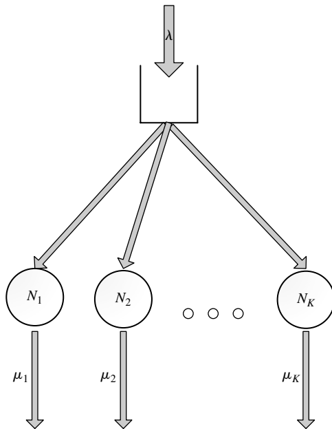
Figure 1 Inverted-V System
