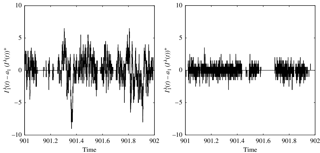
Figure 4 Typical Sample Paths of \{I_1^\lambda(t) - a_1(I^\lambda(t))^+, t \geq 0\} in an Inverted-V System Under the RMI (left) and IR (Right) Policies
