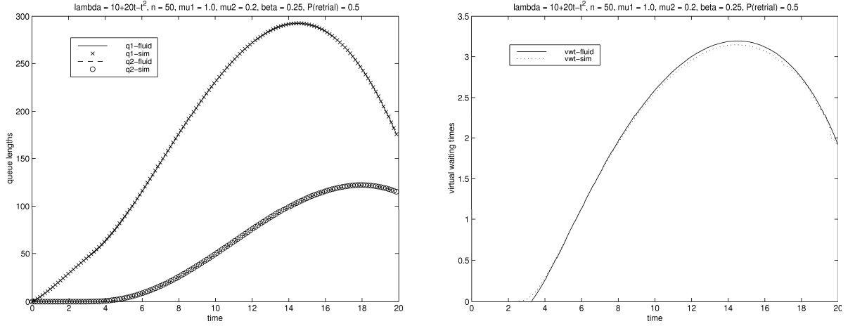
Figure 3: The fluid approximations for the queue lengths and virtual waiting time
