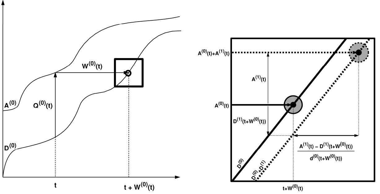
Figure 2: The diffusion term for the attainment waiting time
