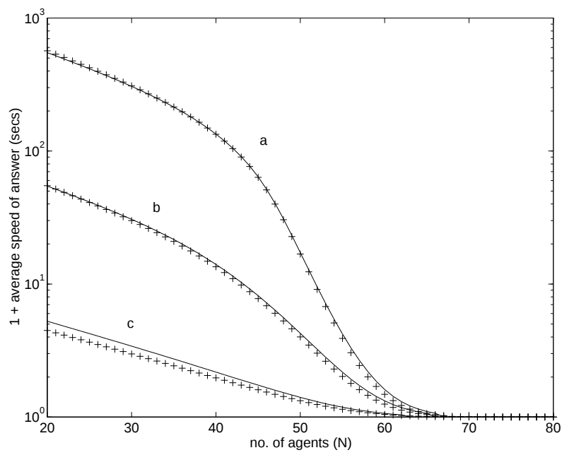
Figure 8: Approximating E[Wait|Served]
