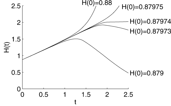
Figure 3. The hazard rate function H(t) for example 1, computed with the myopic equilibrium procedure, for different initial conditions H(0) .
