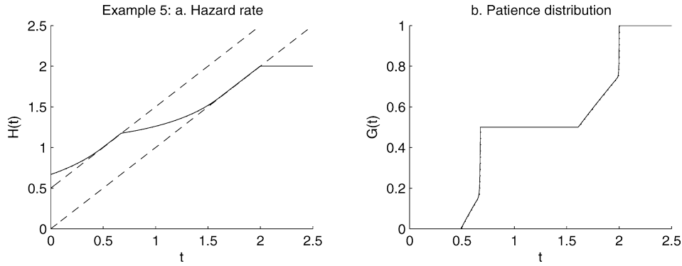
Figure 8. The same perturbed models with \epsilon = 0.01 .
