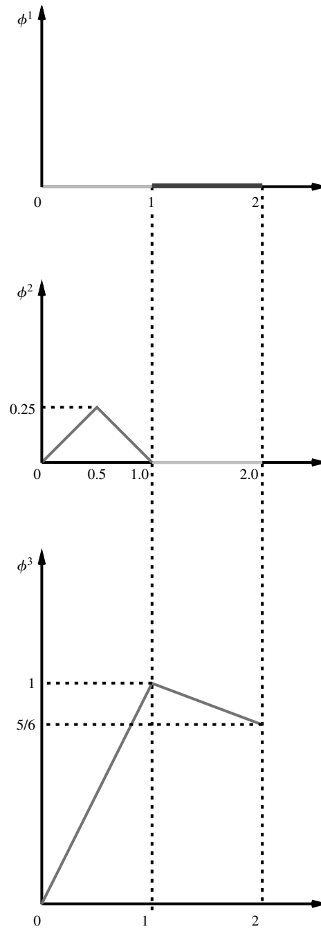
FIGURE 5. The fluid limit of the nonstationary merge queueing network.
