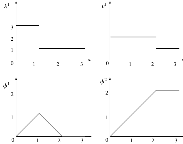
FIGURE 3. The time-varying exogenous arrival rate \lambda^1 to and departure rate \nu^1 from the first queue, along with the contents \phi^1 and \phi^2 of the first and second queue in the tandem network.
